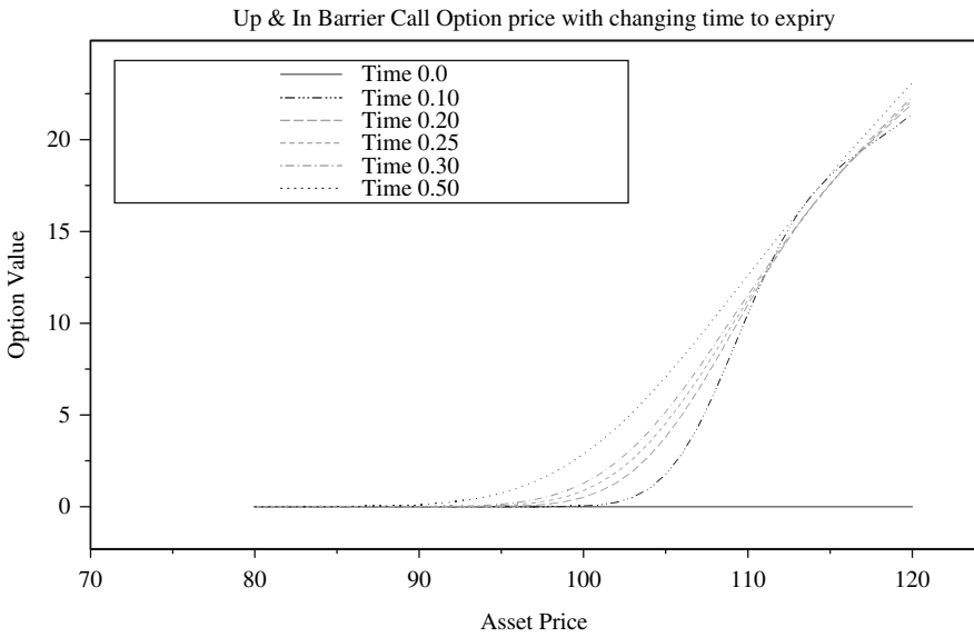
FIGURE 14.2. Up and-in call barrier values for varying times to expiry.
